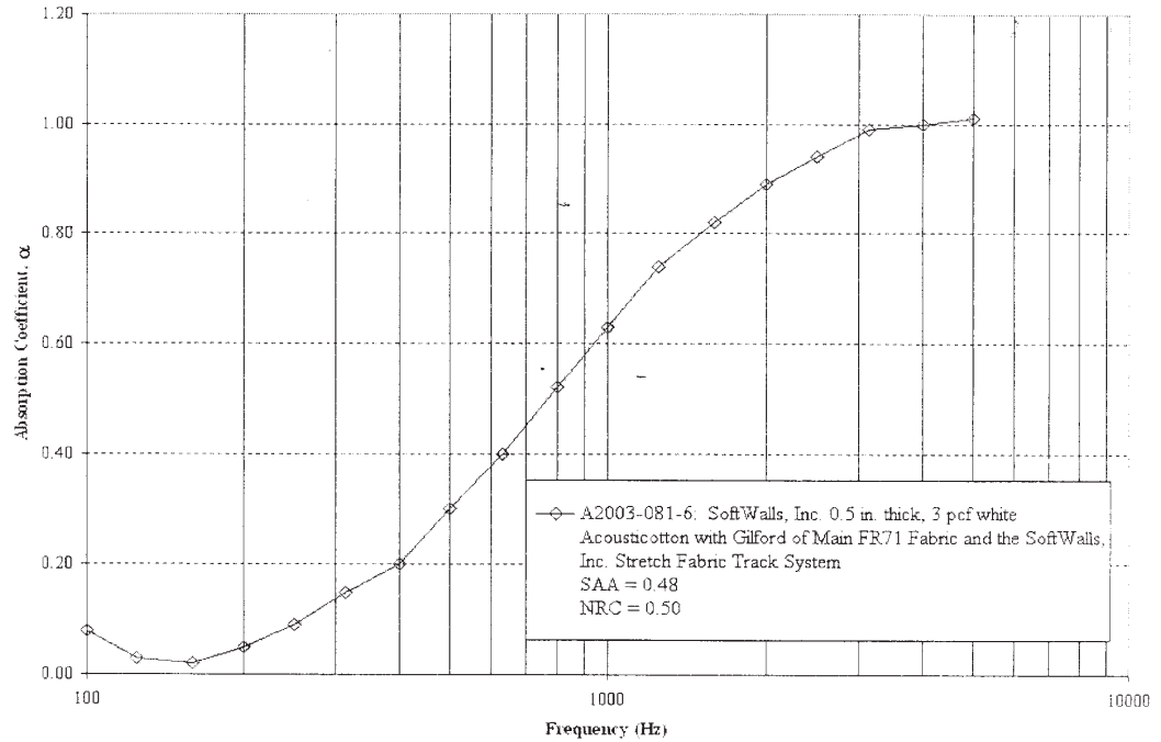
Graph 1. Sound Absorption Performance of SoftWalls, Inc. 0.5 in. thick, 3.0 pcf White Acousticotton with Guilford of Maine FR701 Fabric and the SoftWalls, Inc. Stretch Fabric Track System
